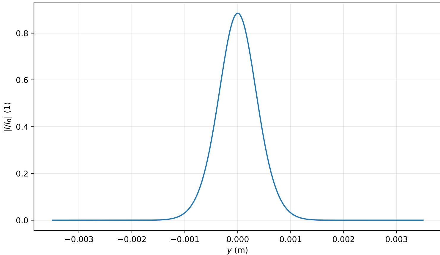
Intensity profile I(x=0, y, z=1.194)/I_0 , \text{Pin}=0.3\text{Pcr} , artificial time
